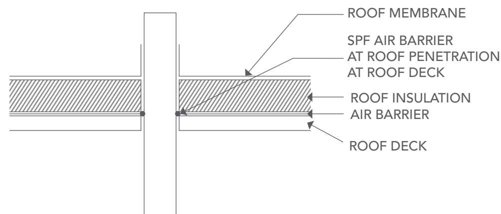
SPF PENETRATION DETAIL: AIR BARRIER BELOW ROOF INSULATION
