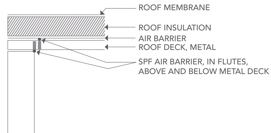
SPF ROOF / WALL INTERSECTION DETAIL: AIR BARRIER BELOW ROOF INSULATION
