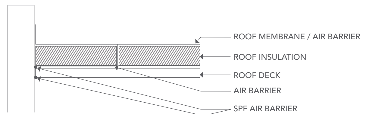
SPF ROOF / WALL INTERSECTION DETAIL: PARAPET WALL
