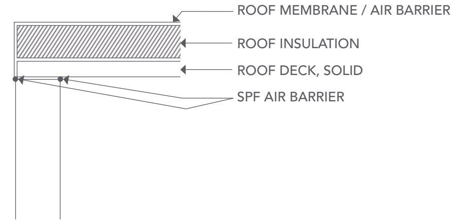
SPF ROOF / WALL INTERSECTION DETAIL: ROOF MEMBRANE AS AIR BARRIER
