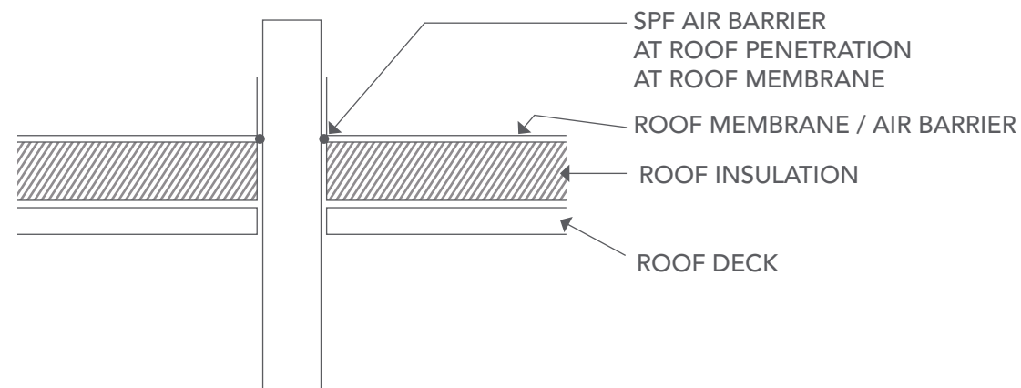
SPF PENETRATION DETAIL: ROOF MEMBRANE AS AIR BARRIER
